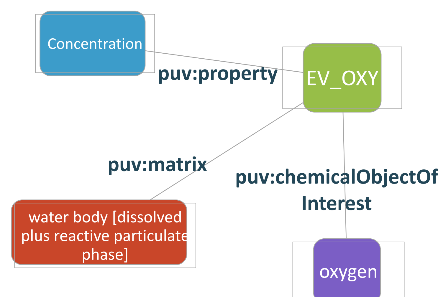
EOV oxygen rules defined using the PUV properties
